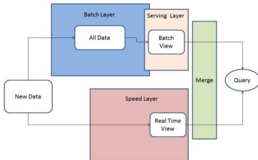
Figure 1: Lambda Architecture
